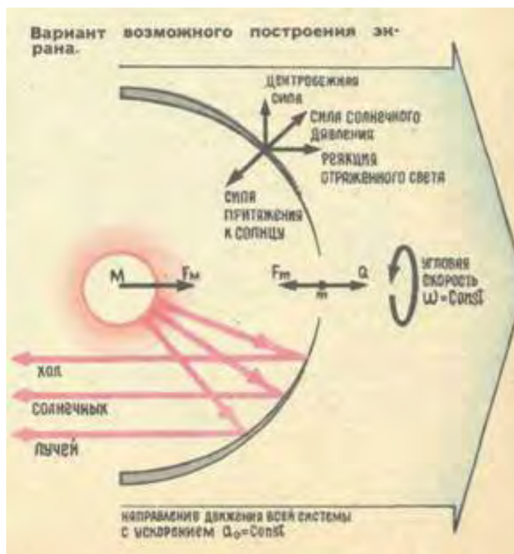
Figure 1 - Shkadov thruster design from TO THE STARS ON ... THE SOLAR SYSTEM , Technology - Youth No. 12 1979, VIKTOR BOROVISHKA, GENNADY SIZENZEV, engineers [1]
